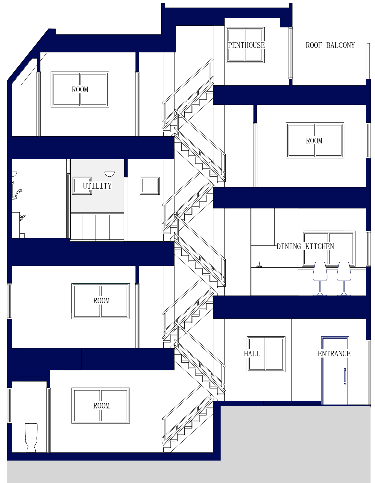
Cross-Section
