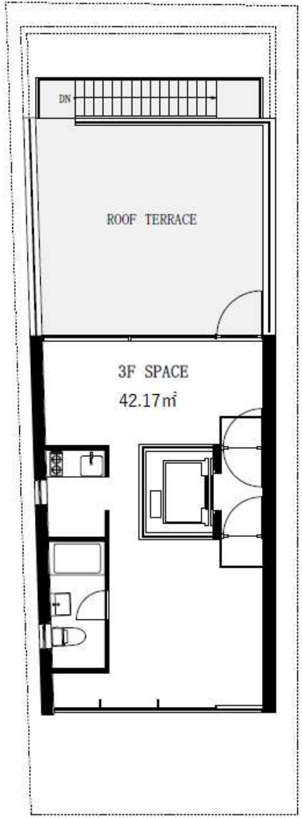
3F PLAN
