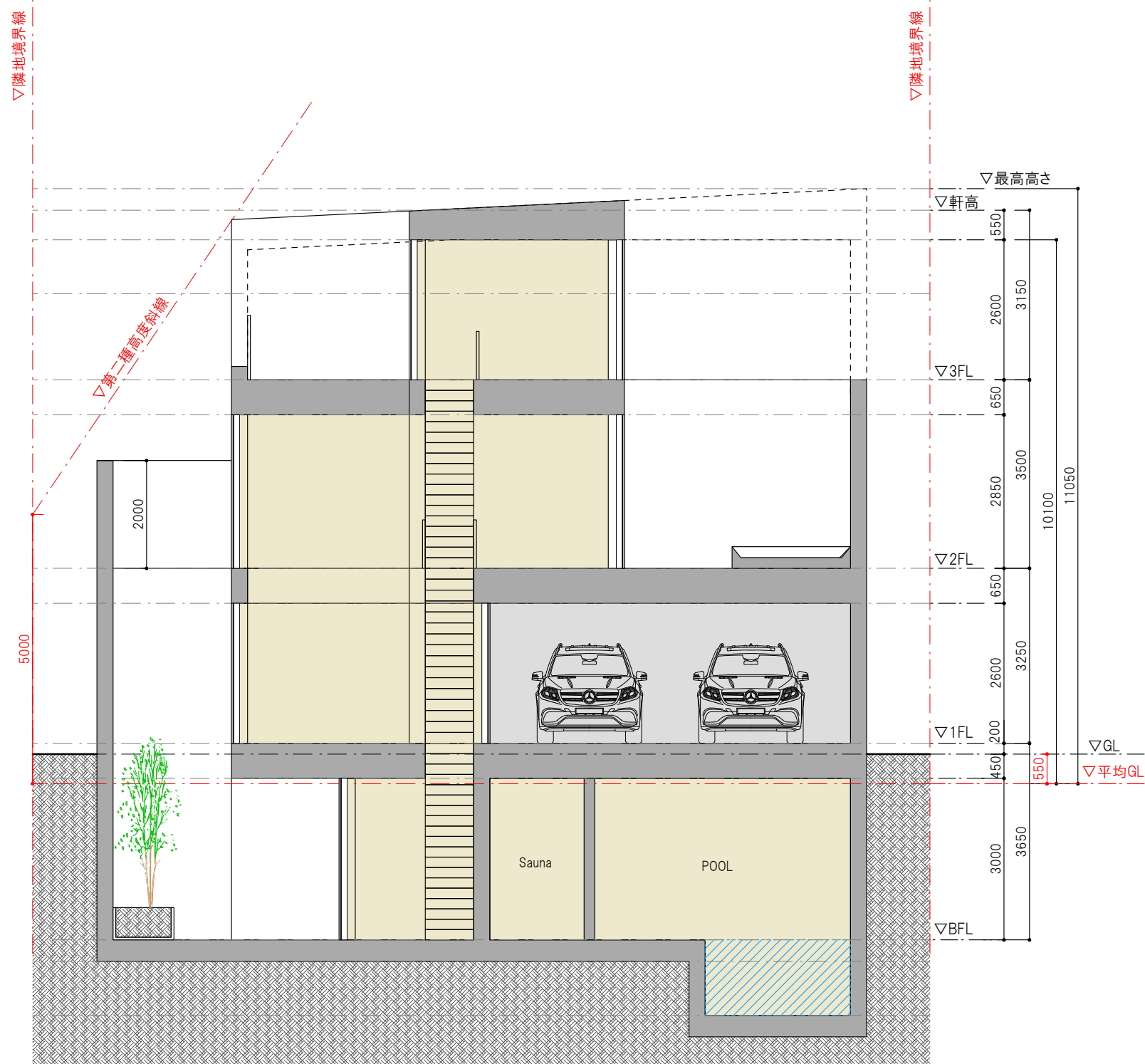
AA' SECTION
