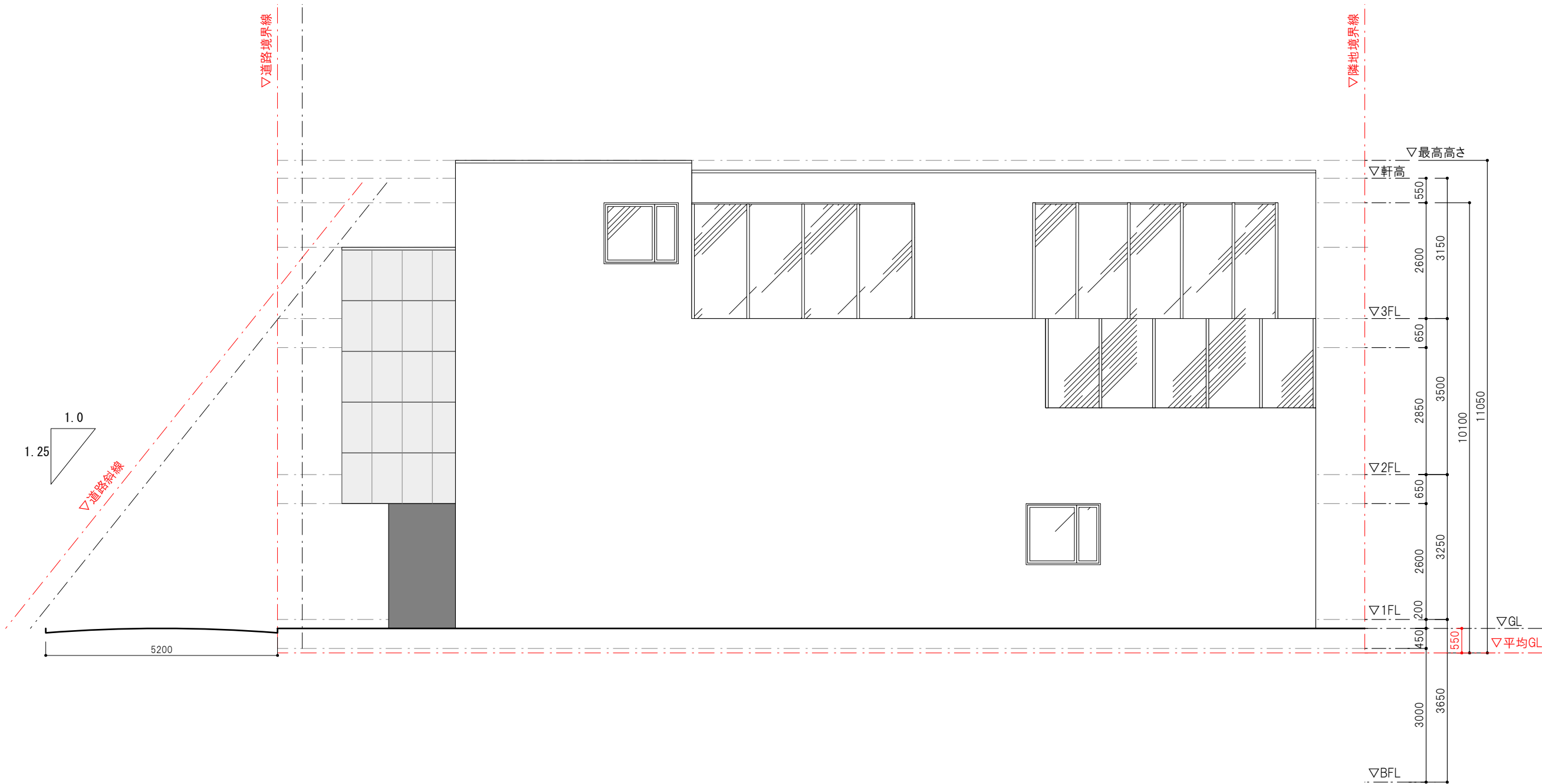
SOUTH ELEVATION
