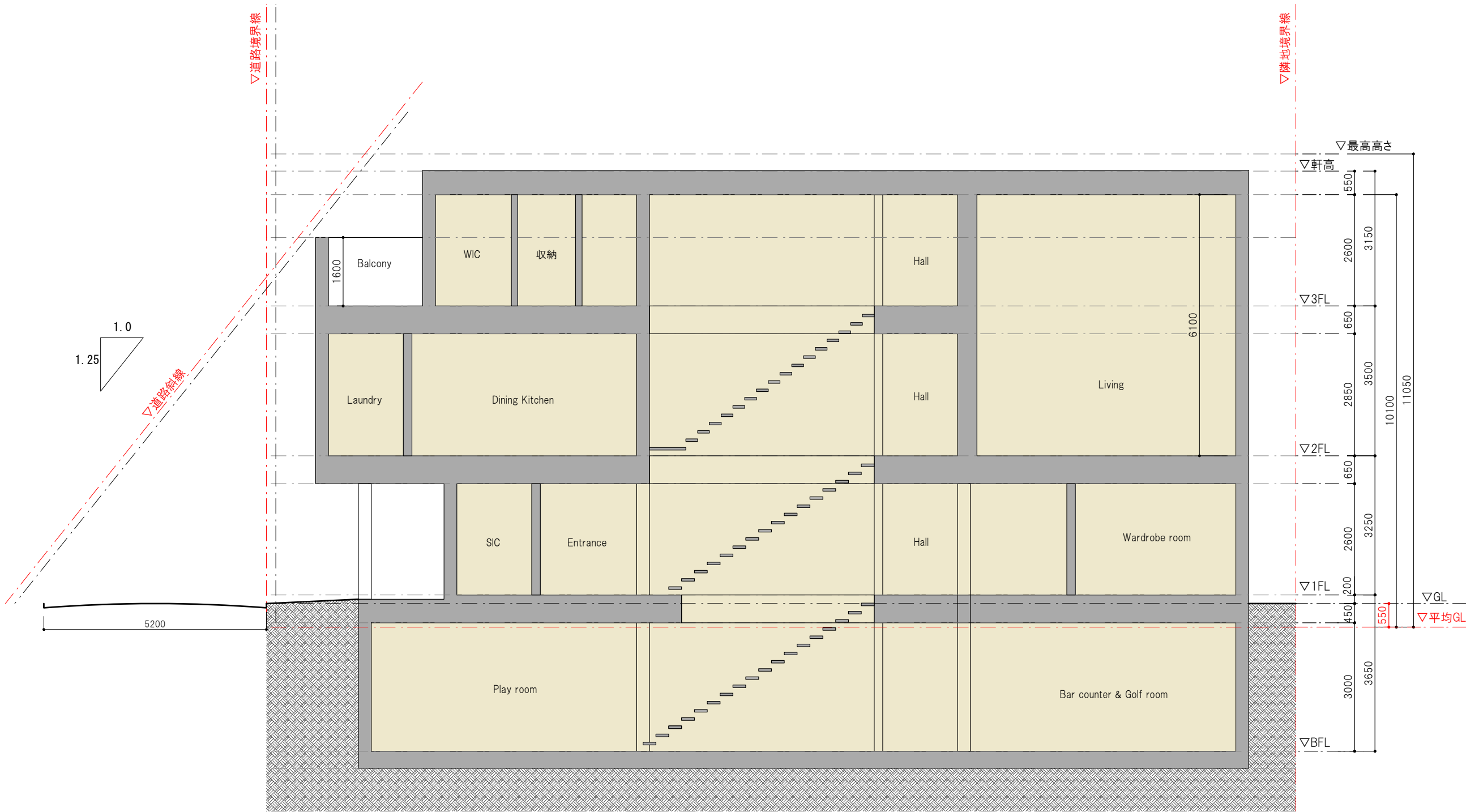
BB' SECTION
