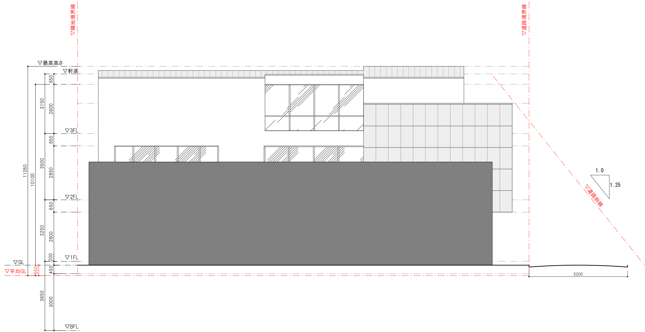
NORTH ELEVATION
